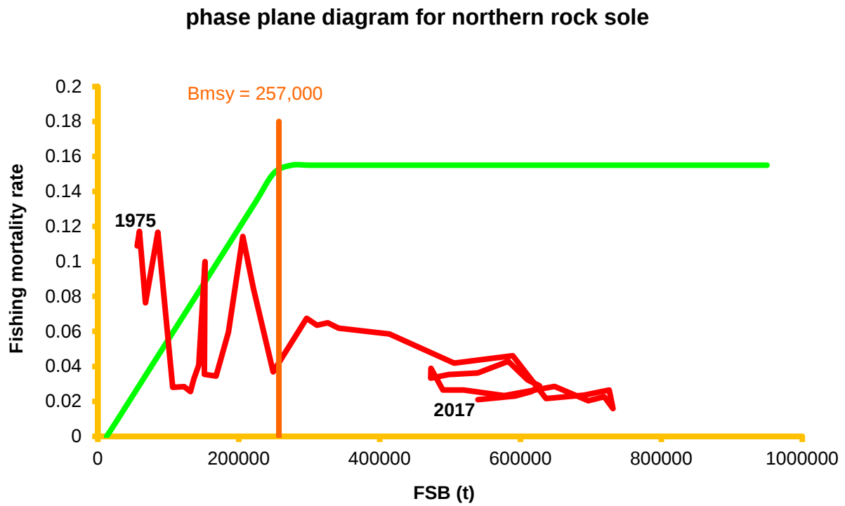
Figure 8.18—Phase-plane diagram of female spawning biomass relative to the harvest control rule.
