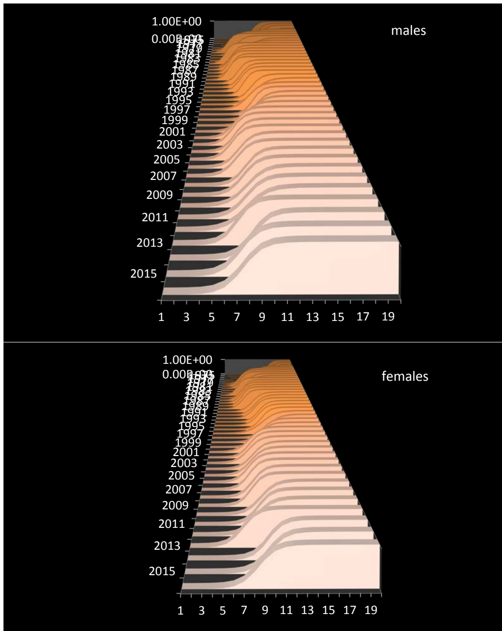
Figure 8.10—Stock assessment model estimates of fishery selectivity at age, by year and gender.
