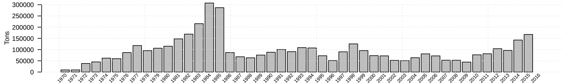
Western, Central, West Yakutat Gulf of Alaska catch of Walleye pollock
