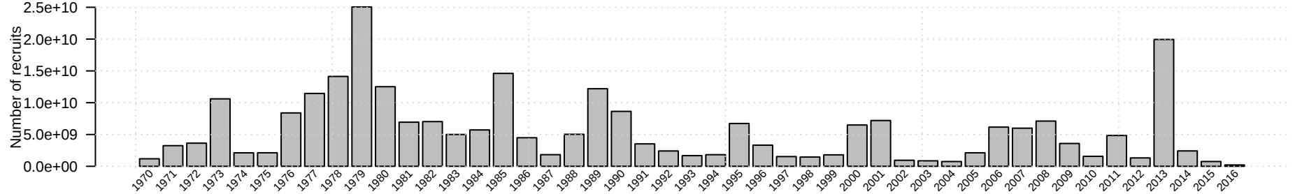
Western, Central, West Yakutat Gulf of Alaska age 1 recruitment of Walleye pollock
