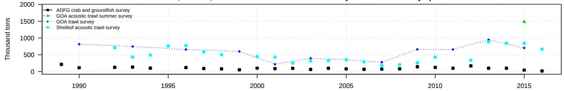
Western, Central, West Yakutat Gulf of Alaska survey biomass of Walleye pollock
