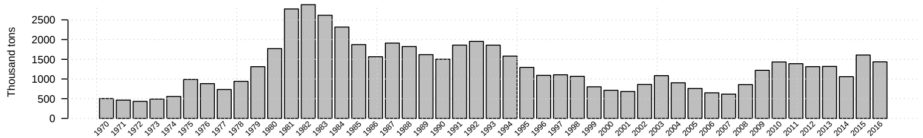
Western, Central, West Yakutat Gulf of Alaska age 3 plus biomass of Walleye pollock
