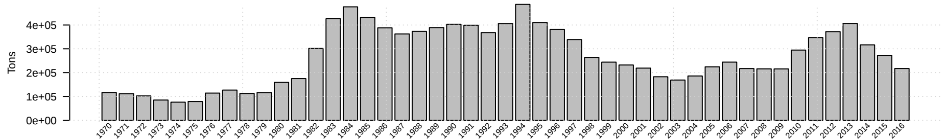
Western, Central, West Yakutat Gulf of Alaska spawning biomass of Walleye pollock
